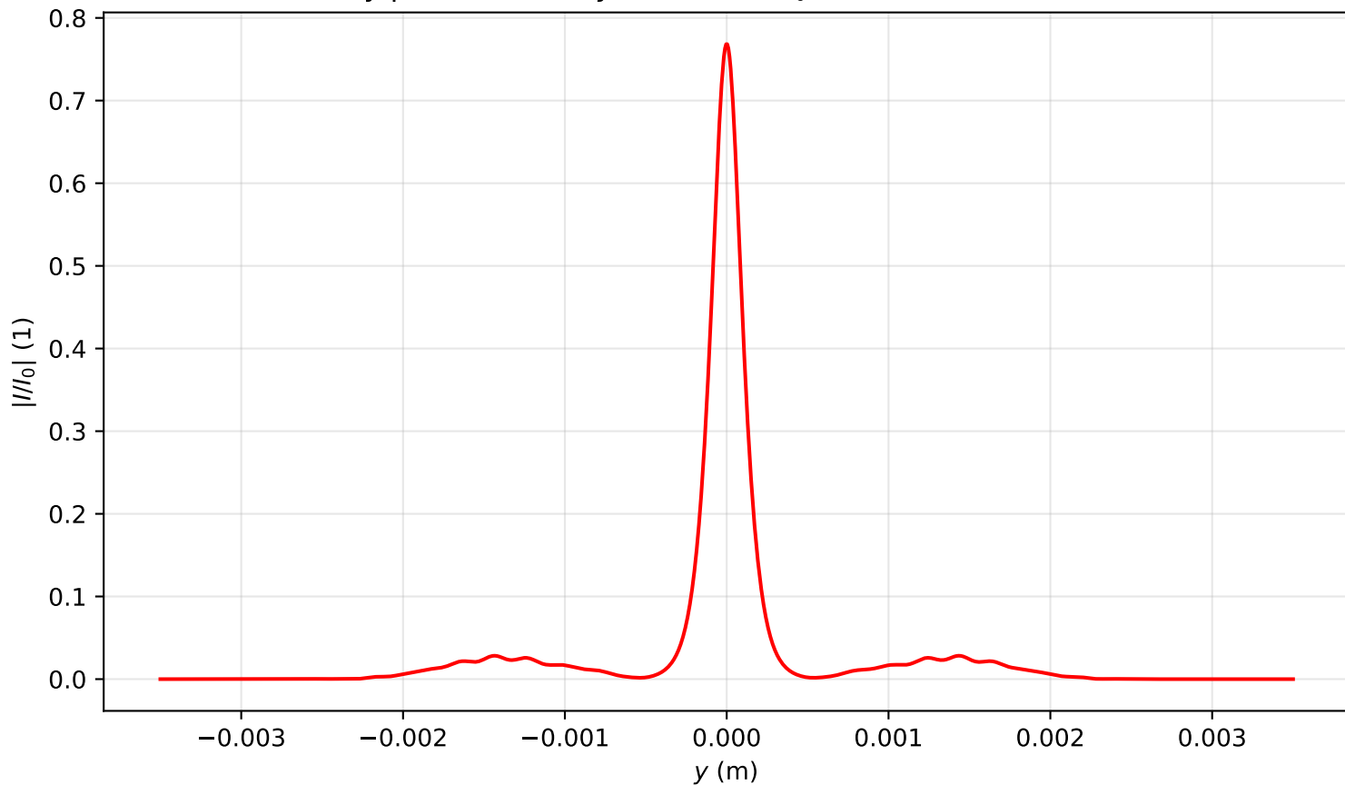
Intensity profile I(x=0, y, z=1.433)/I_0 , \text{Pin}=9.0\text{Pcr} , artificial time
